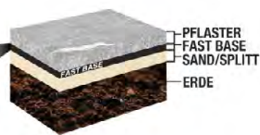
FAST BASE Methode
